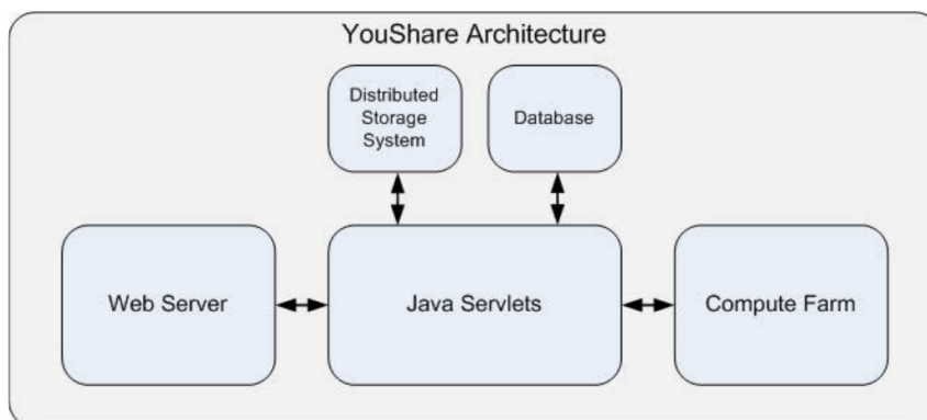
Figure 14: Overview of the YouShare architecture.
